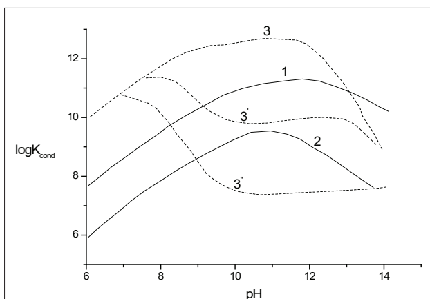
Figura 4. Dependenta \log K^{\text{cond}} de pH.
