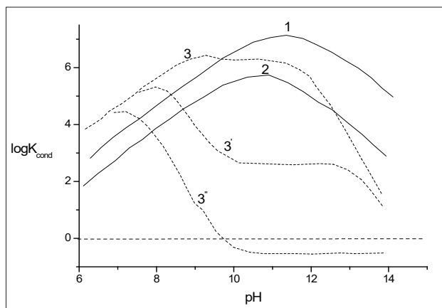
Figura 3. Dependenta \log K^{\text{cond}} de pH.
