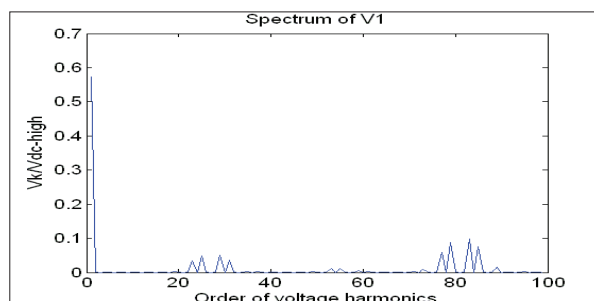
Figure 19. Pole voltages V_{iH} and V_{iL} , line voltages V_{1H2H} and V_{1L2L} , and phase voltage V_1 (with its spectrum) of PV system with continuous synchronous PWM ( F=50\text{Hz} , F_s=1.35\text{kHz} , V_H=V_L , m_H=m_L=0.45 ) [14].
