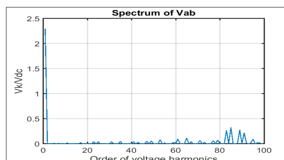
Figure 14. Line voltages, and spectrum of the V_{ab} voltage, of modular converter on the base of standard inverters with continuous synchronous PWM (CPWM, F=35\text{Hz} , m=0.7 ) [8].
