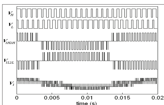
Figure 19. Pole voltages V_{iH} and V_{iL} , line voltages V_{1H2H} and V_{1L2L} , and phase voltage V_1 (with its spectrum) of PV system with continuous synchronous PWM ( F=50\text{Hz} , F_s=1.35\text{kHz} , V_H=V_L , m_H=m_L=0.45 ) [14].
